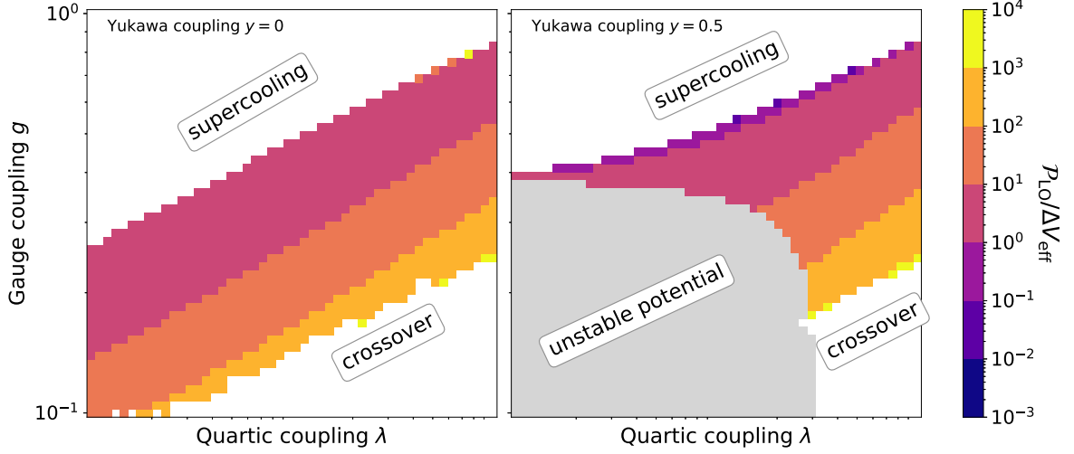
Figure 13: The leading-order friction \mathcal{P}_{LO} over the difference \Delta V_{eff} in potential energy between the true and false vacuum phases as a function of the quartic coupling \lambda and the gauge coupling g for values of the Yukawa coupling y = 0 and y = 0.5 . Values greater than one indicate that relativistic bubble wall velocities cannot be reached, cf. eq. (A.1). For values smaller than one, a relativistic terminal velocity is expected.
